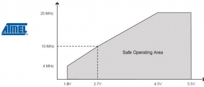
Figure 28-1. Maximum Frequency vs. V_{CC}
