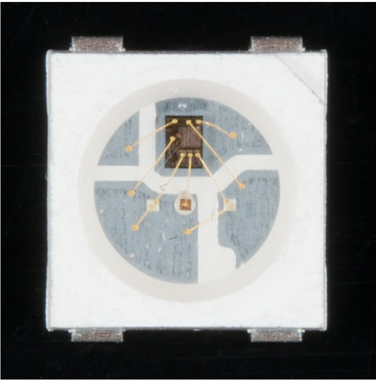
Addressable WS2812B Close Up
